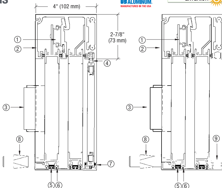
DW Series Window With Screen
