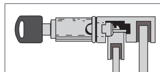
Typical Keyed Lock Installation
