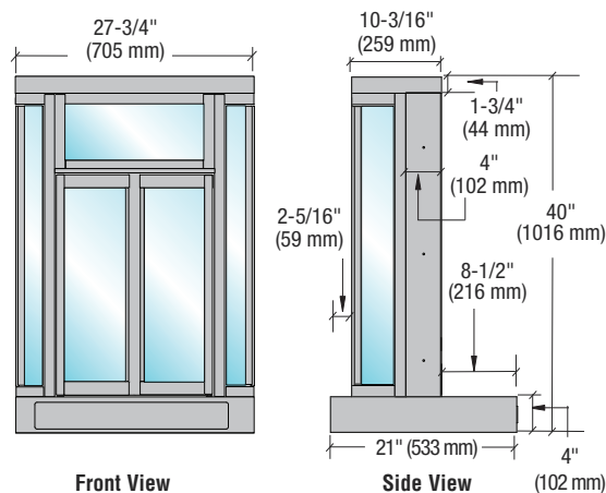
Projected Manual Model (Viewed from Clerk's Side)
