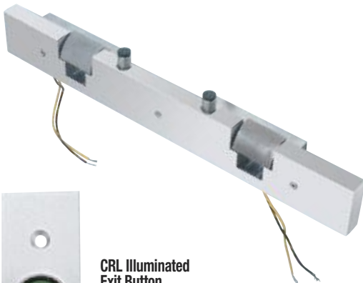
CRL Electric Strike Keeper for Double Doors
