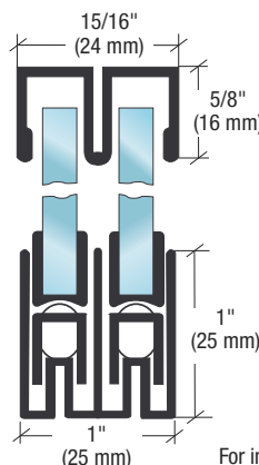
Ball Bearing Carrier
