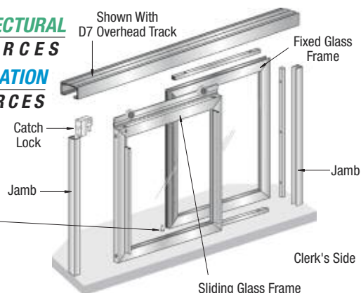
Spring-Loaded Guide
