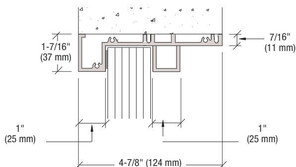
Standard Inset Aluminum
