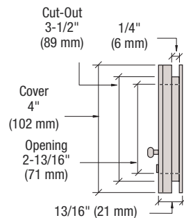
4" (102 mm) Model Requires 3-1/2" (89 mm) Hole
