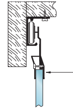
Standard Assembly: D8A Single Overhead Track D679 Rollers D28A Front Hanger
