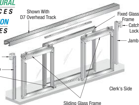
Spring-Loaded Guide
