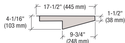
Unit Side View
