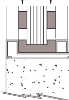
Full Frame Option
