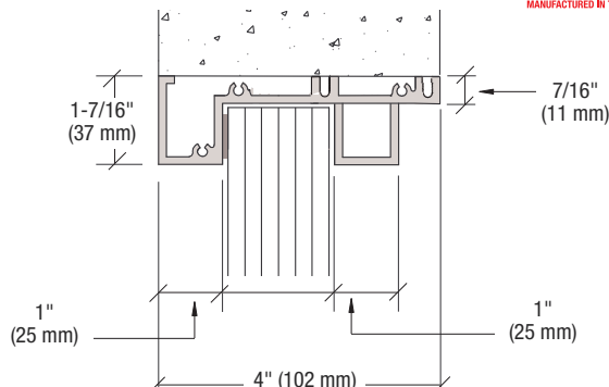
Narrow Inset Aluminum
