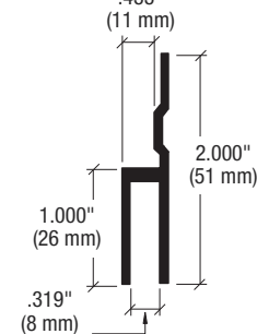
D41 Rear Hanger
