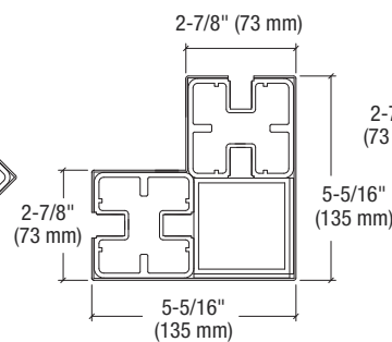
Surface Mount Post Stanchions
