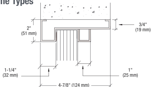
Standard Inset Stainless
