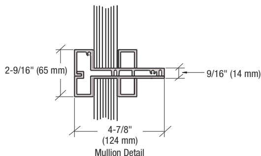
Mullion Detail
