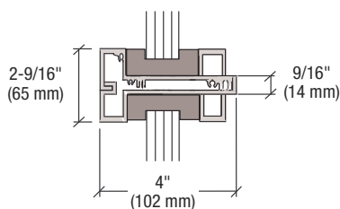
Mullion Detail
