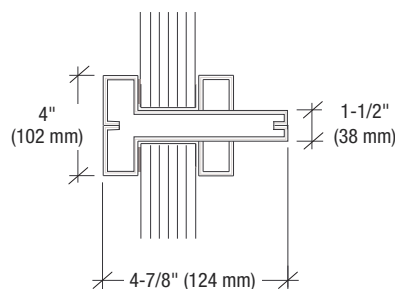
Mullion Detail
