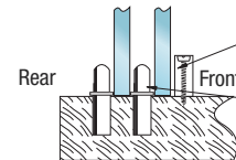
D30 Nylon Guides used to prevent removal of doors by tilting to the front. D35 Spring Loaded Guides used when frequent removal of doors is required.
