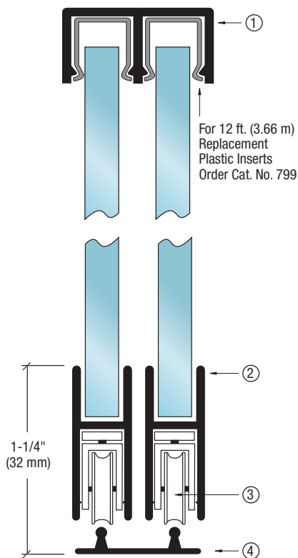
CAT. NO. DV147 Nylon Wheel Assembly (12)
