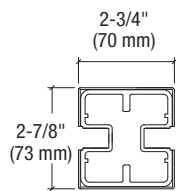
Vertical Posts
