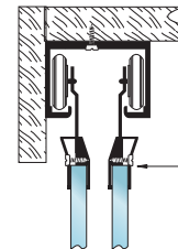
Standard Assembly: D6A Overhead Track D679 Rollers D28A Front Hangers Both Sides
