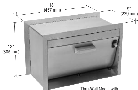
Thru-Wall Model with 1" (25 mm) Flanges (Clerk's Side Shown) Both Flanges are Adjustable
