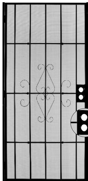
Frame Size 3/4" (19 mm) x 3/4" (19 mm)
