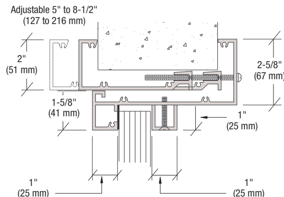
Clamp-On Aluminum
