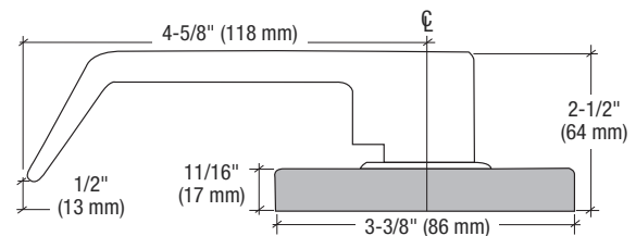
Classroom Function (F 84)
