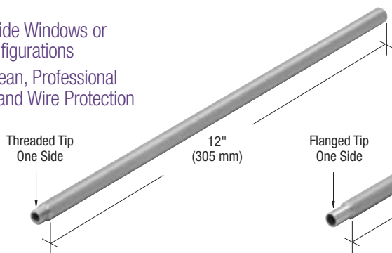
MODEL 9C0NT 3/8" (10 mm) Diameter Straight Tube With Threaded Tip
