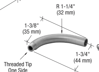
MODEL 9C0NE 3/8" (10 mm) Diameter 90 Degree Elbow Tube With Threaded Tip
