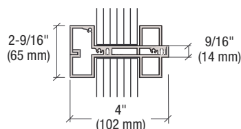
Mullion Detail
