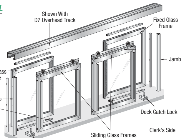
Spring-Loaded Guide
