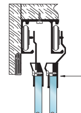
Standard Assembly: D9A Double Overhead Track D679 Rollers D28A Front Hanger D29A Rear Hanger
