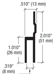
D40 Front Hanger
