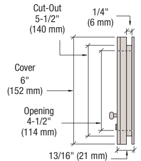
6" (152 mm) Model Requires 5-1/2" (140 mm) Hole
