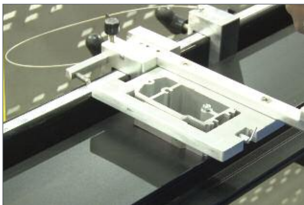
Shear Block Locator shown with Shear Block, which is purchased separately
