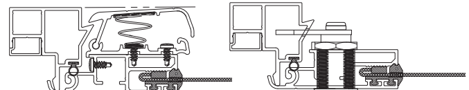
Quick Escape Security Window Screen Cross Section
