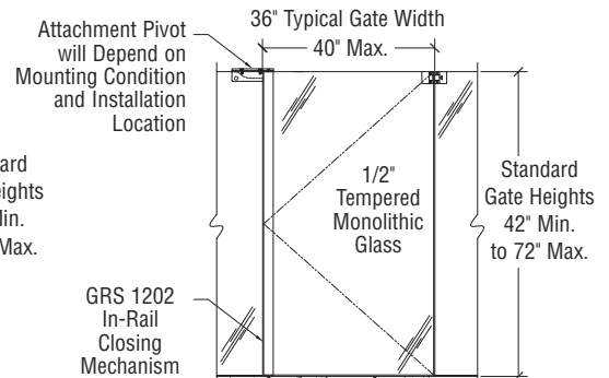
Glass Mount Application
