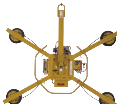
Manual Rotator/Tilter
