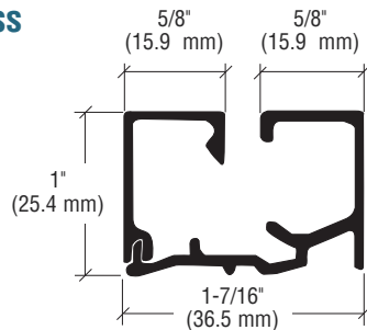
Two-Piece Snap-In Sash
