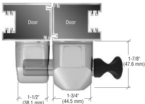
Plan View: Face Mount Lock
