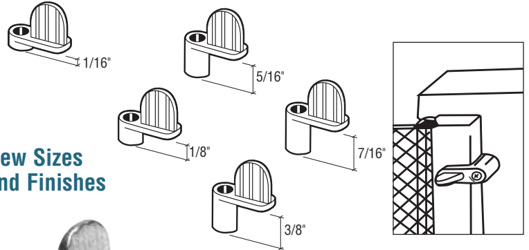
Typical Applications for Window Screen Clips
