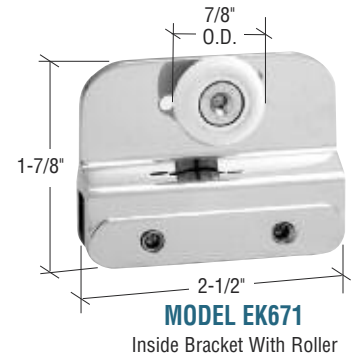
Inside Bracket With Roller
