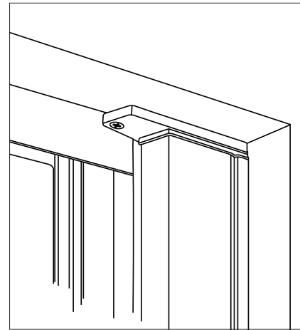
Internal Mounting
