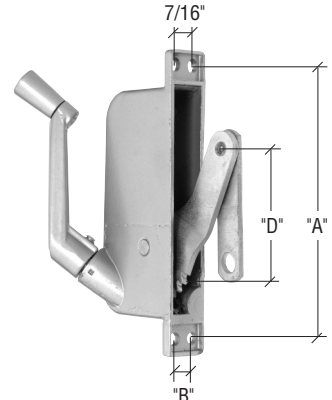
Type IV Housing 2 Top Holes 2 Bottom Holes
