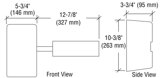
ECL230D-Short Bar (Cylinder and bar guard sold separately)
