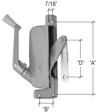
Type I Housing 2 Top Holes 2 Bottom Holes With Offset
