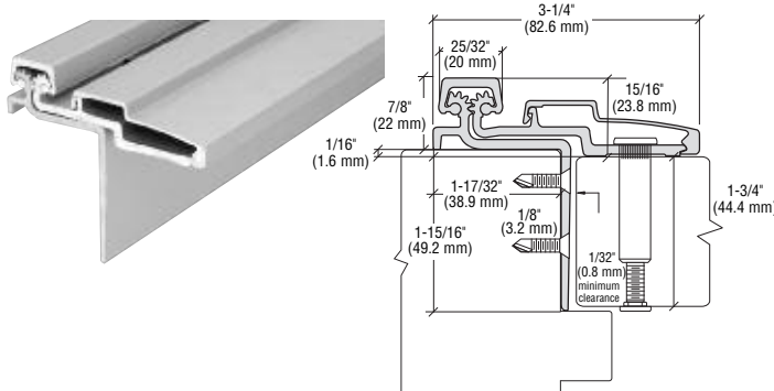
HEAVY-DUTY HALF SURFACE/FRAME LEAF CONTINUOUS HINGES
