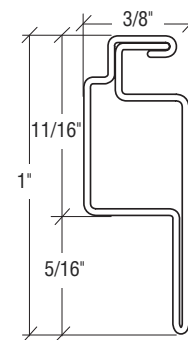
WSC117 Mitered Corners See page 155W
