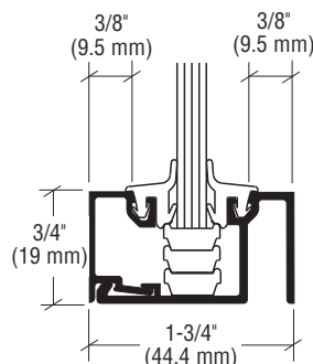
Two-Piece Transom Sash
