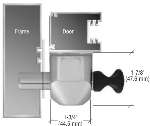
Plan View: Side Mount Lock
