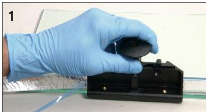
Apply Super Spacer® to clean glass surface with SSNH or SSAPA as release liner is removed.
