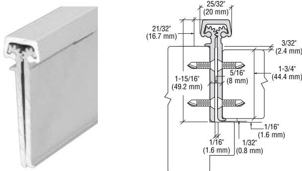
STANDARD DUTY CONCEALED LEAF CONTINUOUS HINGES
