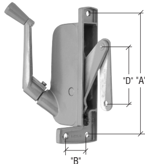
Type II Housing 1 Top Hole 2 Bottom Holes With Offset
