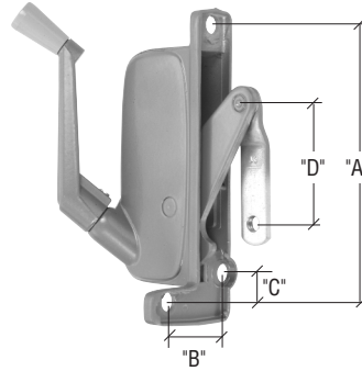
Type III Housing 1 Top Hole; 1 Side Hole 1 Bottom Hole With Offset
