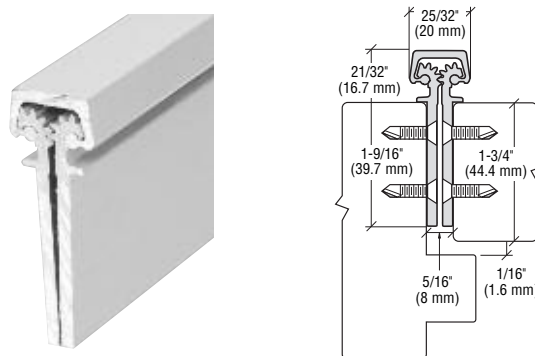
STANDARD DUTY CONCEALED LEAF CONTINUOUS HINGES
