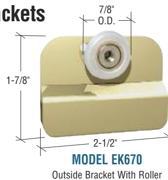
Outside Bracket With Roller
