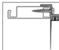
Typical Installation on Roll-Formed Door
