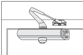
Regular Projecting Arm Installation
