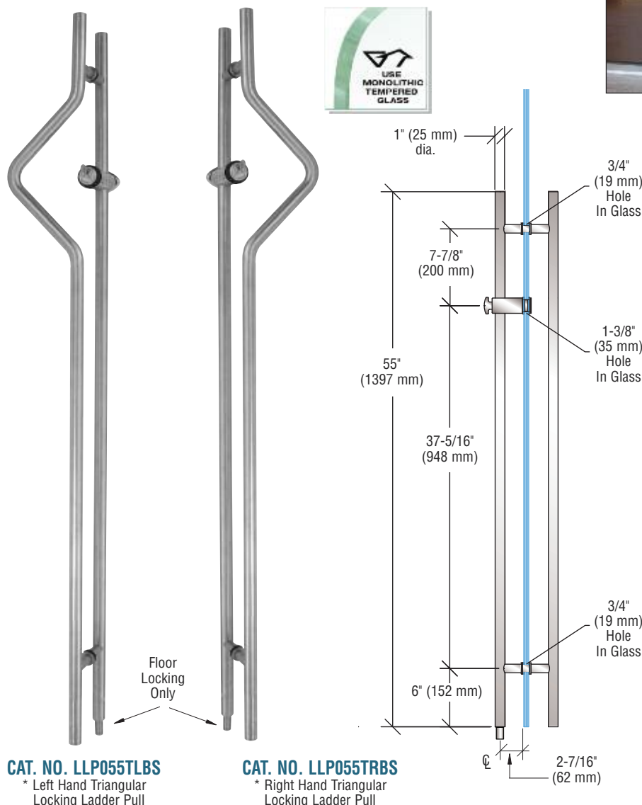
Single Door Installation With Right Hand Locking Ladder Pull
