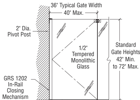
Wall/Flat Post Mount Application
