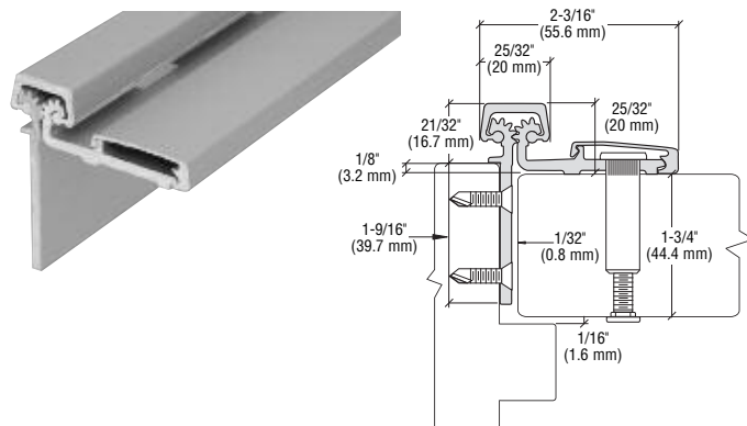
STANDARD DUTY HALF SURFACE CONTINUOUS HINGES
