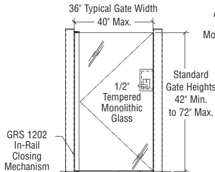
Round Post Mount Application
