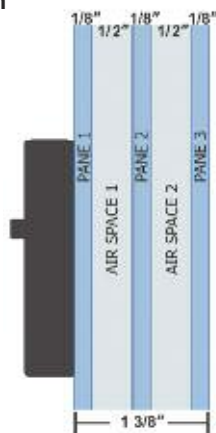
Total Thickness Triple Pane Window
