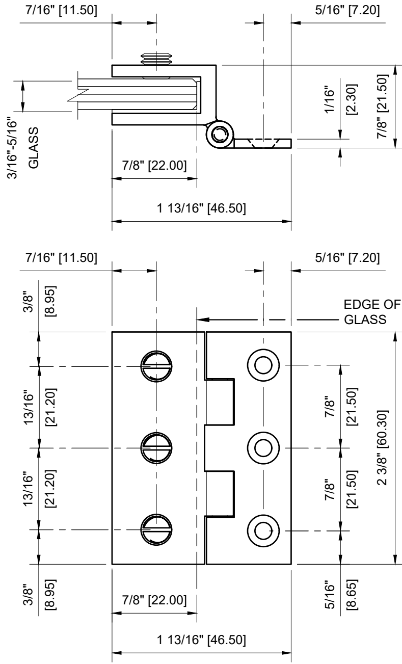
CRL - EH169 LARGE 2-3/8" WALL MOUNT HINGE FOR 3/16" - 5/16" GLASS
