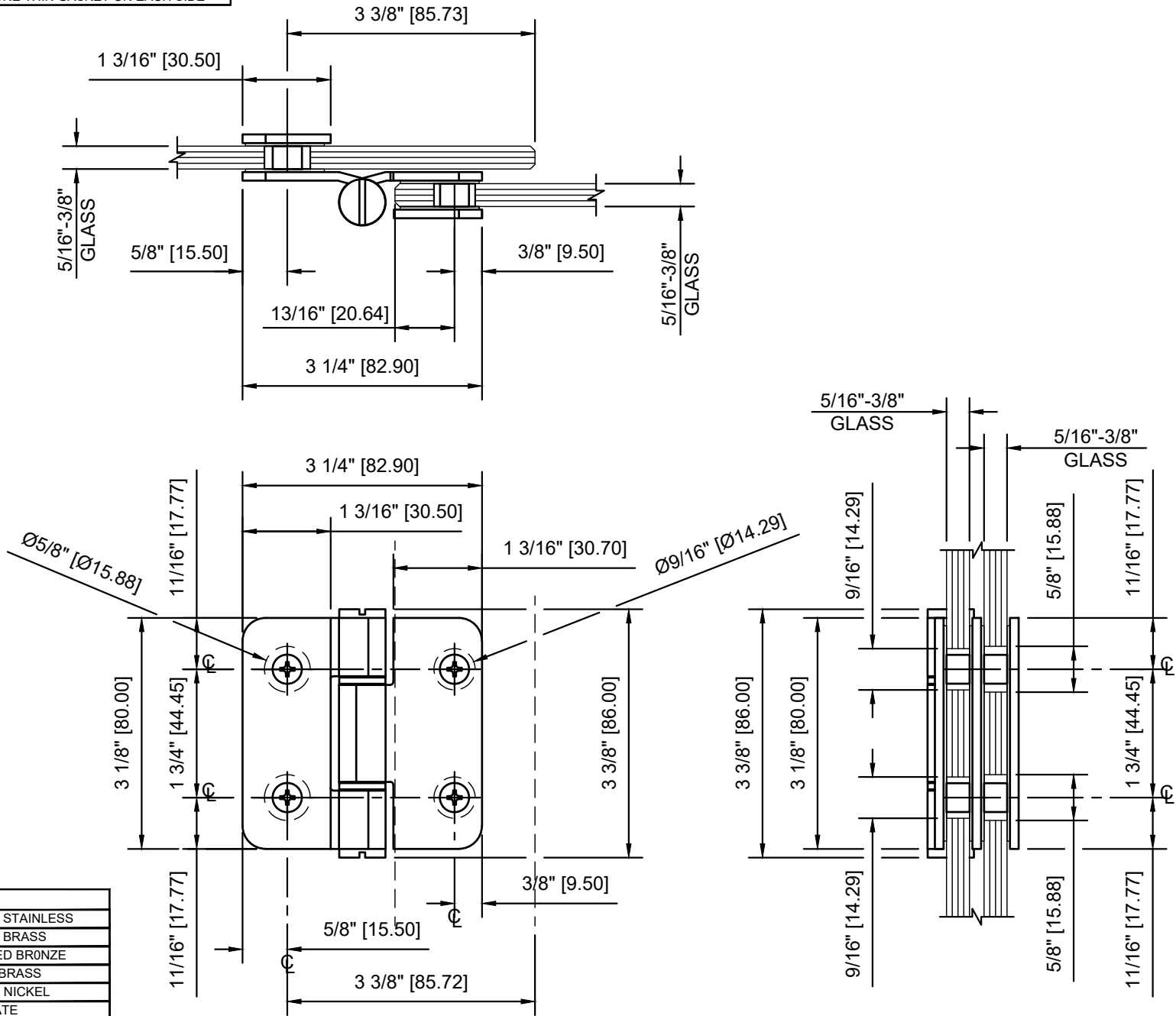
ZUR01XX - CRL ZURICH SERIES GLASS TO GLASS MOUNT BI-FOLD HINGE
