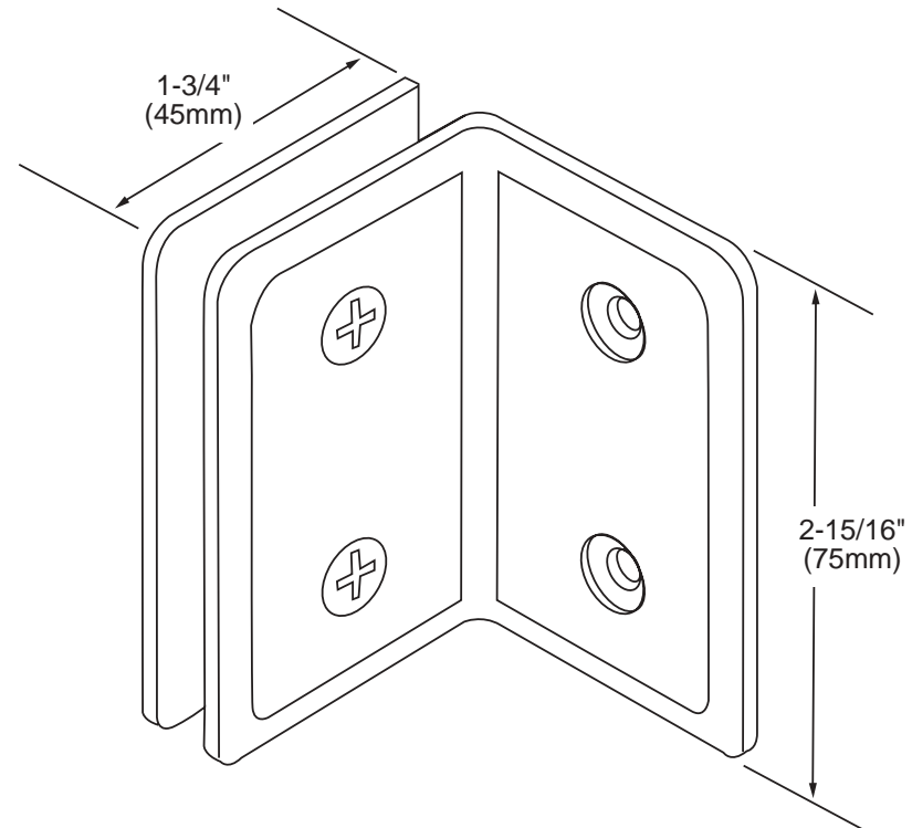
REAR VIEW
